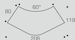
120° SYMMETRICAL DESK
