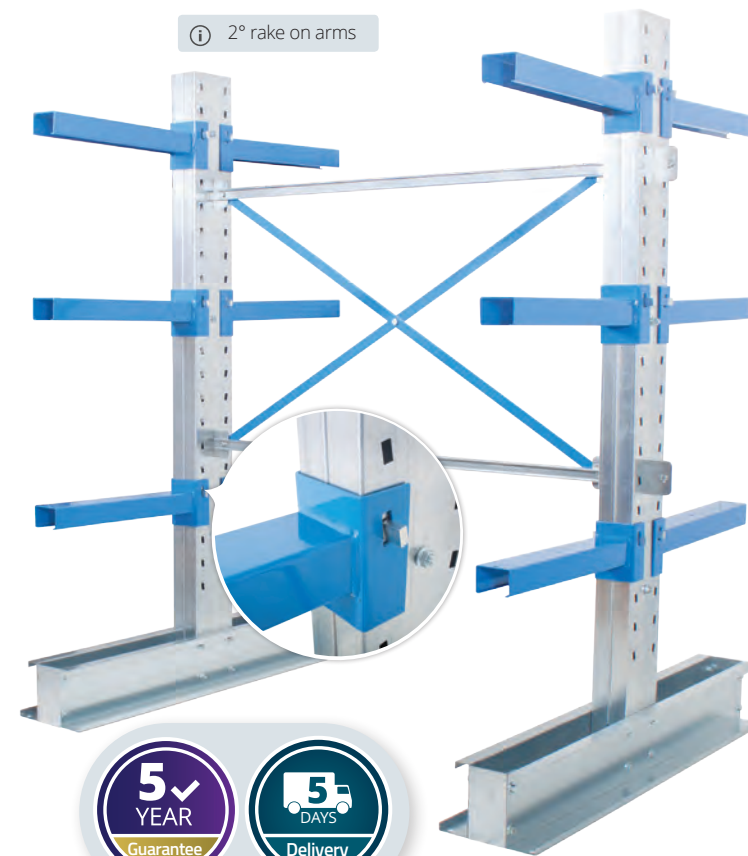
Double Sided Cantilever Rack 1976 x 1500 x 600 +detail on arm attached to the column
