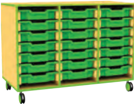
7 High Triple Bay H756 x W1021 x D494 mm
