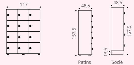
Lockers with 12 compartments on screw feet - front view
