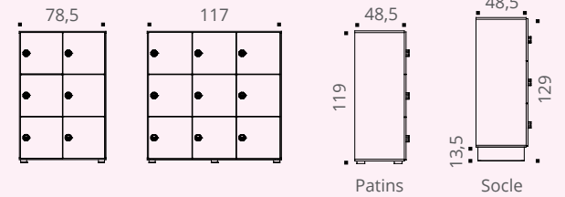
Lockers with 6 / 9 compartments on screw feet - front view
